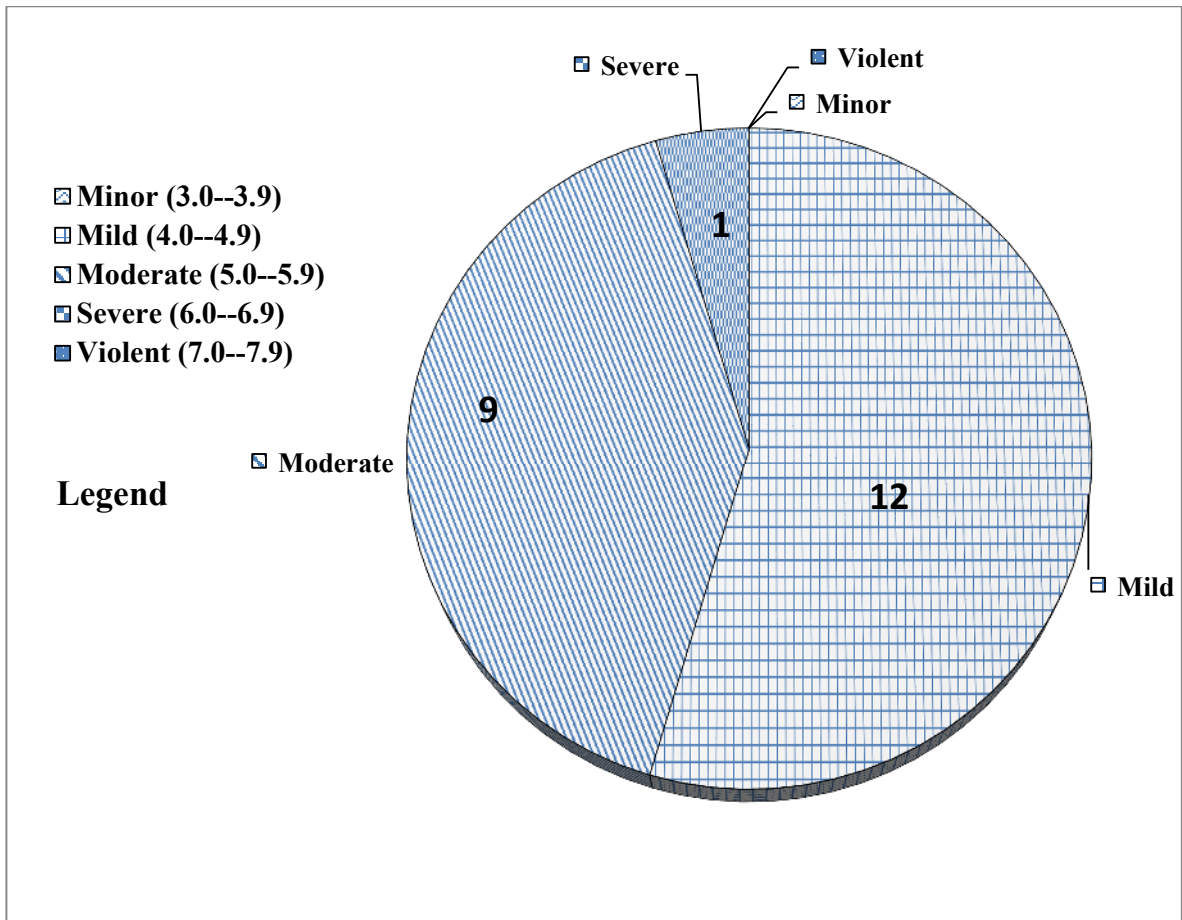
Figure 1: Frequency Analysis of the Magnitude of the Seismic Events Recorded by PMD Seismic Network. It shows the number of events recorded during the month of May, 2022 for different categories of severity.
