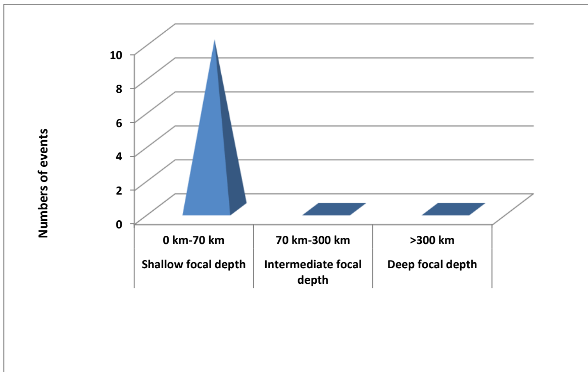
Figure2: Analysis of major earthquakes based on focal depth during the month of May, 2022.
