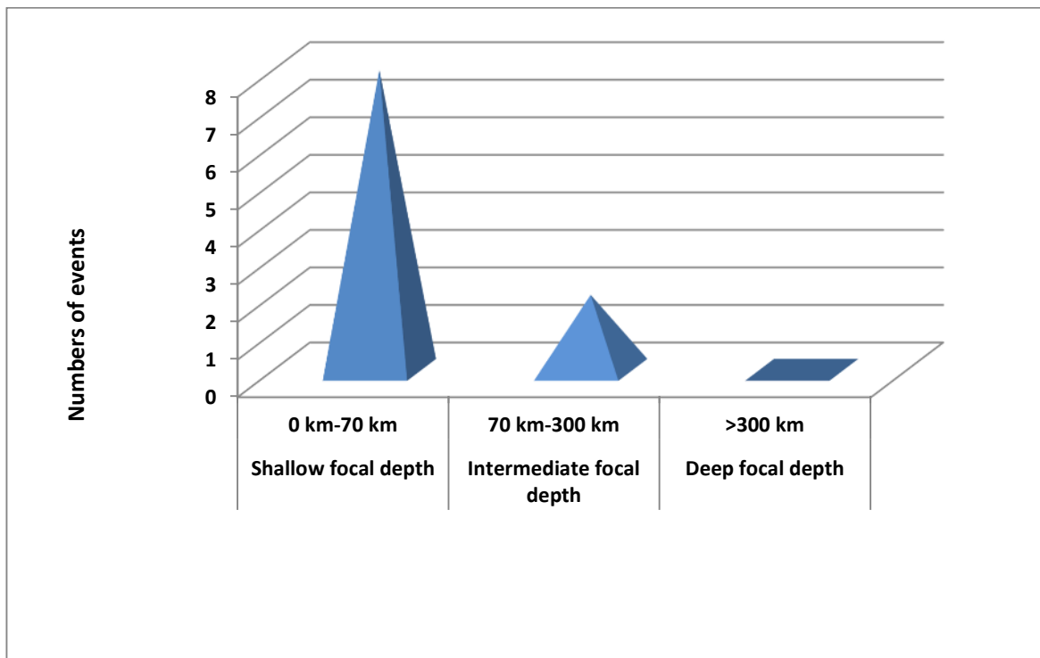
Figure2: Analysis of major earthquakes based on focal depth during the month of March, 2022.
