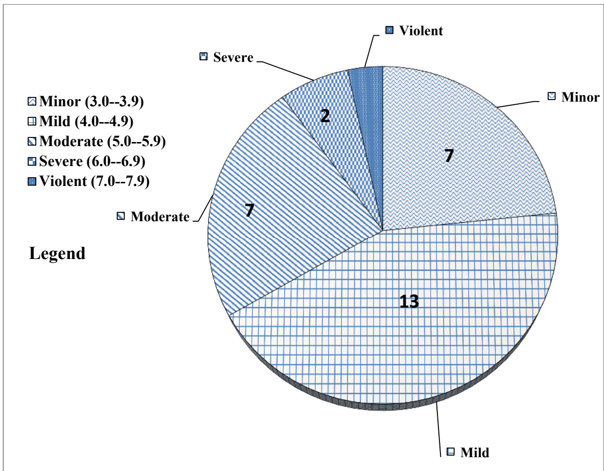
Figure 1: Frequency Analysis of the Magnitude of the Seismic Events Recorded by PMD Seismic Network. It shows the number of events recorded during the month of March, 2022 for different categories of severity.
