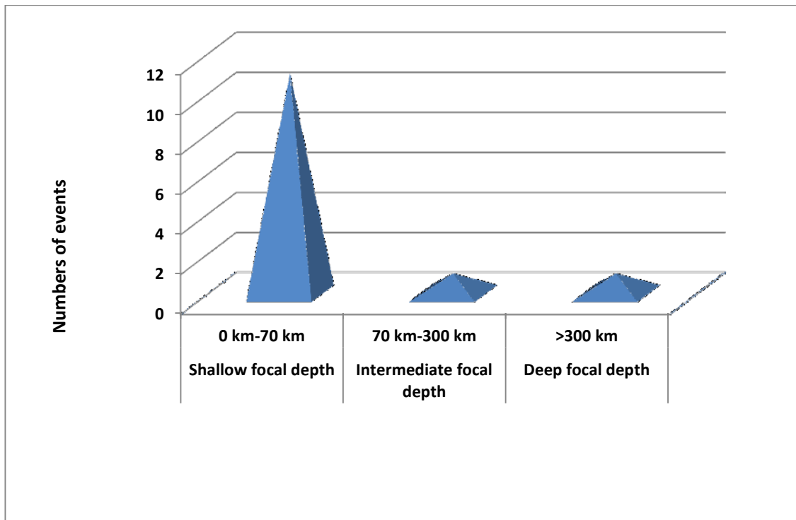
Figure2: Analysis of major earthquakes based on focal depth during the month of January, 2022.
