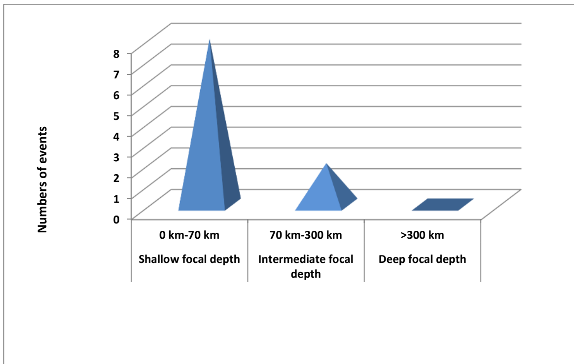
Figure2: Analysis of major earthquakes based on focal depth during the month of April, 2022.
