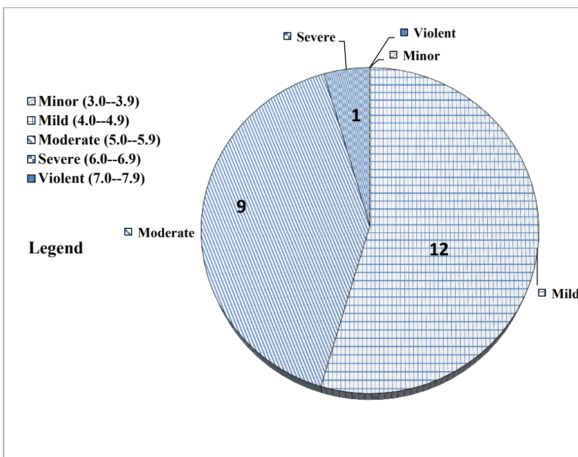
Figure 1: Frequency Analysis of the Magnitude of the Seismic Events Recorded by PMD Seismic Network. It shows the number of events recorded during the month of April, 2022 for different categories of severity.
