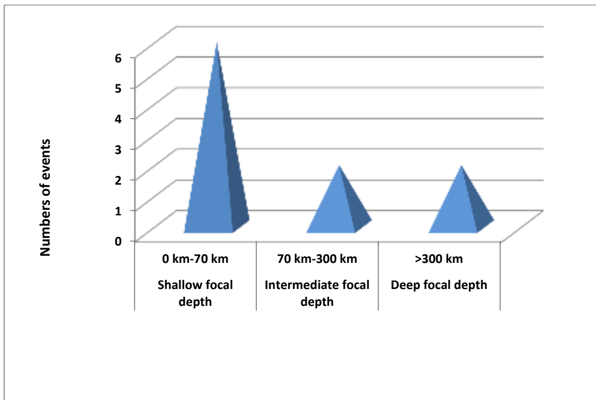
Figure2: Analysis of major earthquakes based on focal depth during the month of September, 2021.
