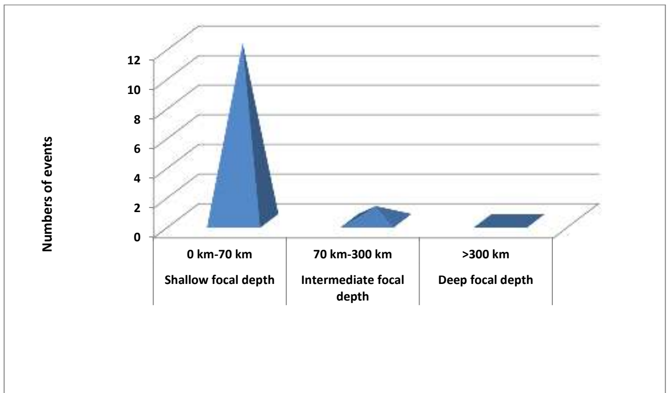
Figure2: Analysis of major earthquakes based on focal depth during the month of March, 2021.
