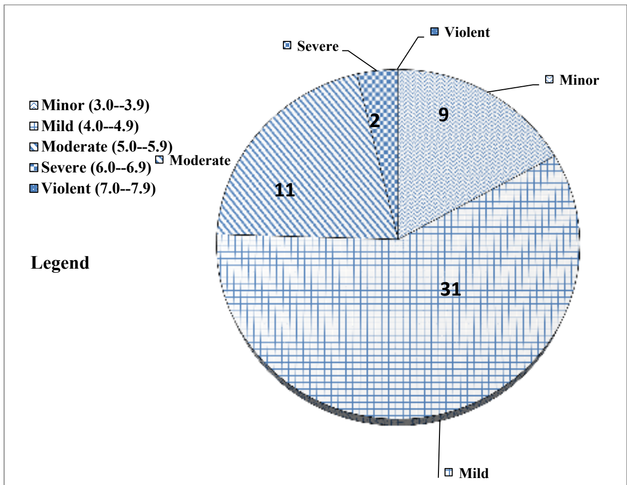
Figure01: shows the number of events recorded during the month of March, 2021 for different categories of severity.
