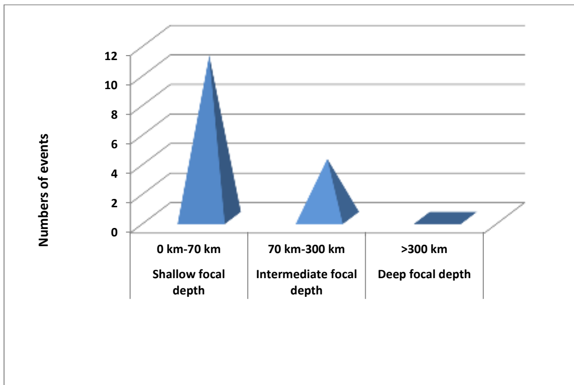
Figure2: Analysis of major earthquakes based on focal depth during the month of June, 2021.
