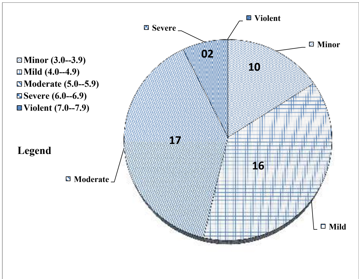
Figure01: shows the number of events recorded during the month of January, 2021 for different categories of severity.
