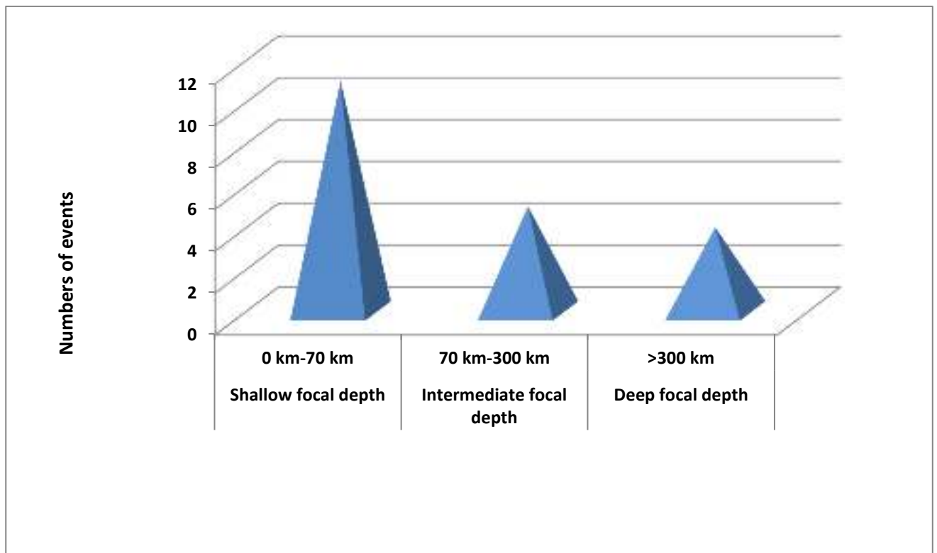
Figure2: Frequency analysis of major earthquakes based on focal depth during the month of January, 2021.
