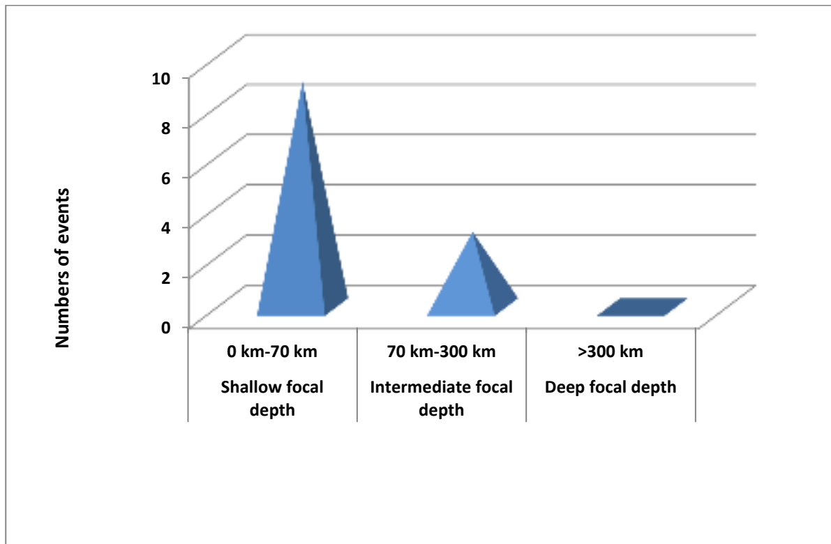
Figure2: Analysis of major earthquakes based on focal depth during the month of August, 2021.
