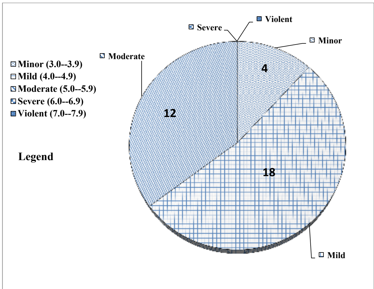
Figure01: shows the number of events recorded during the month of August, 2021 for different categories of severity.
