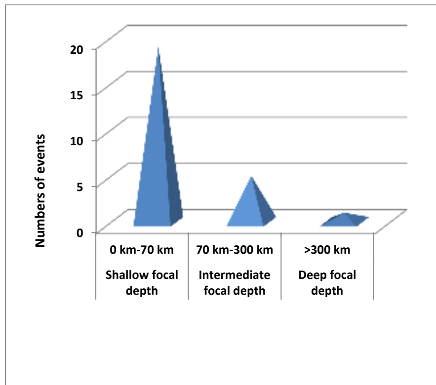
Figure2: Frequency analysis of major earthquakes based on focal depth during the month of September, 2020.
