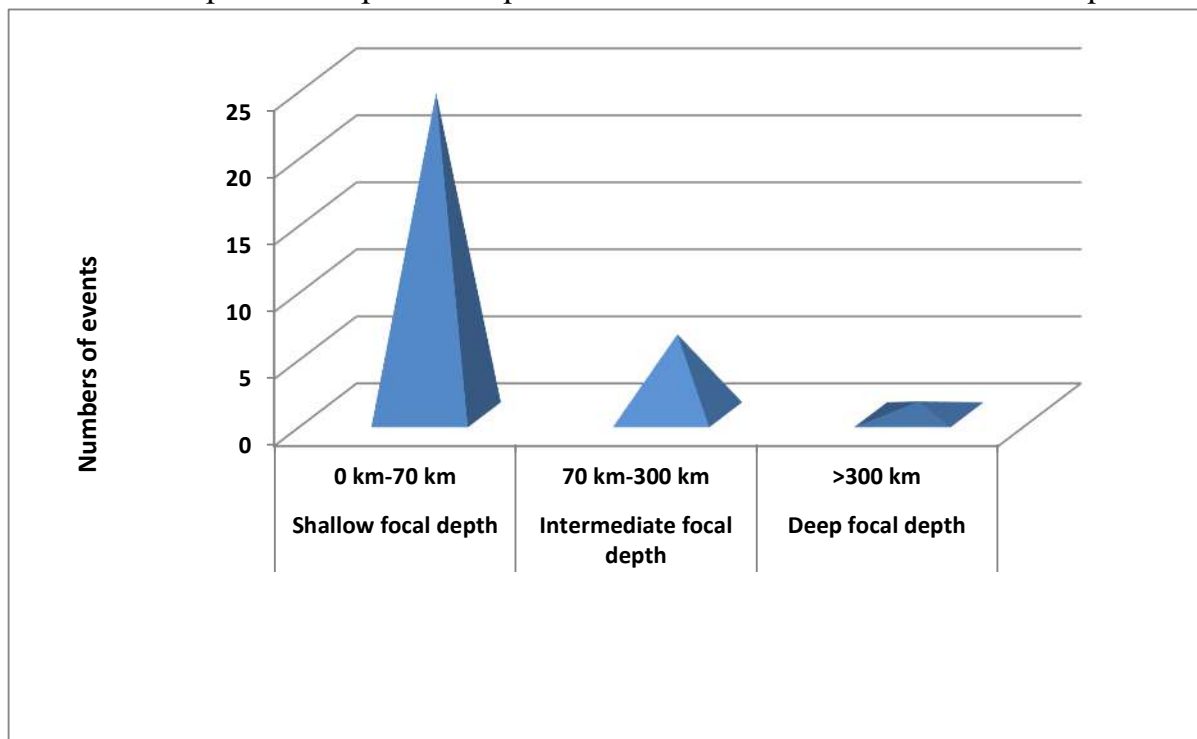
Figure2: Frequency analysis of major earthquakes based on focal depth during the month of May, 2020.
