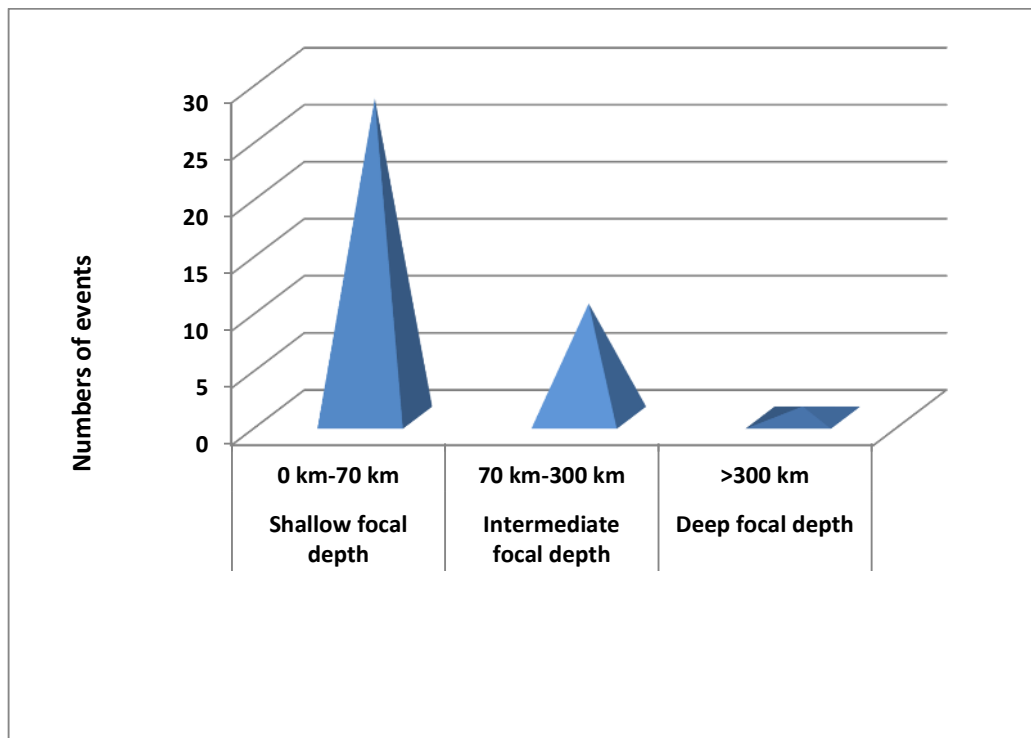
Figure2: Frequency analysis of major earthquakes based on focal depth during the month of June, 2020.
