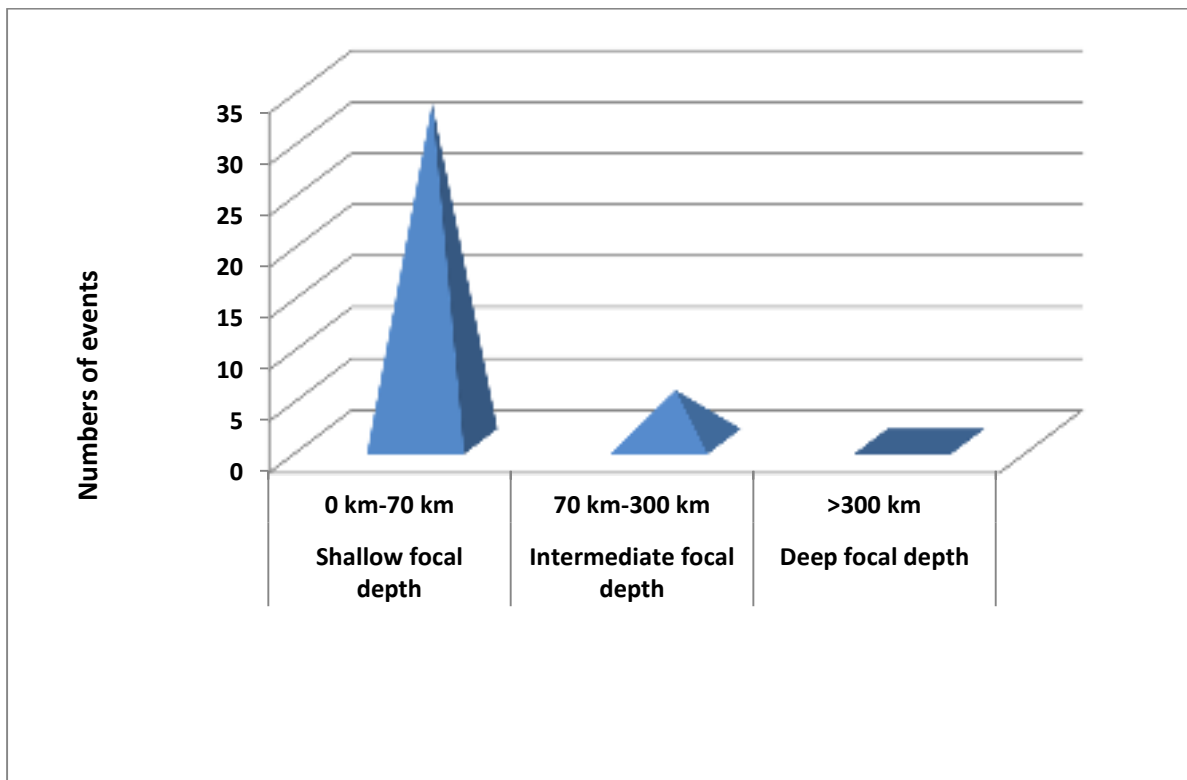
Figure2: Frequency analysis of major earthquakes based on focal depth during the month of January, 2020.
