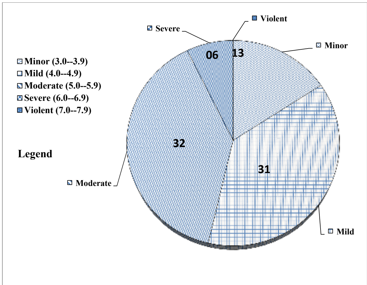
Figure01: shows the number of events recorded during the month of January, 2020 for different categories of severity.
