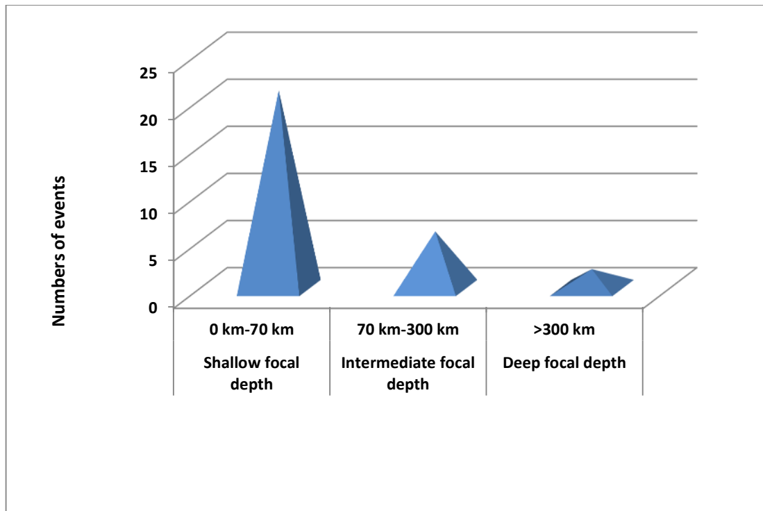
Figure2: Frequency analysis of major earthquakes based on focal depth during the month of February, 2020.
