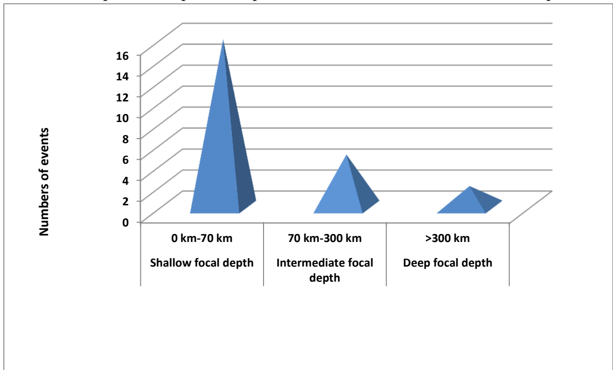
Figure2: Frequency analysis of major earthquakes based on focal depth during the month of April, 2020.
