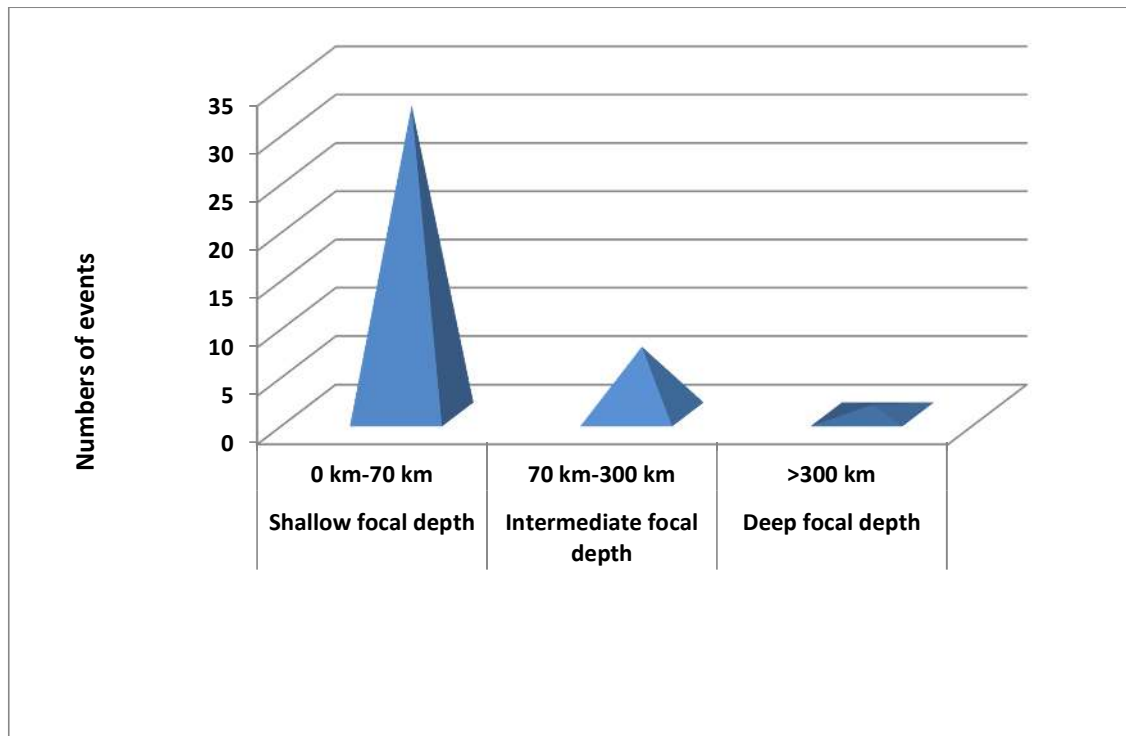
Figure2: Frequency analysis of major earthquakes based on focal depth during the month of November, 2019.
