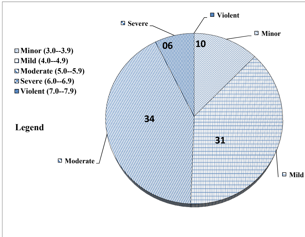
Figure01: shows the number of events recorded during the month of November, 2019 for different categories of severity.
