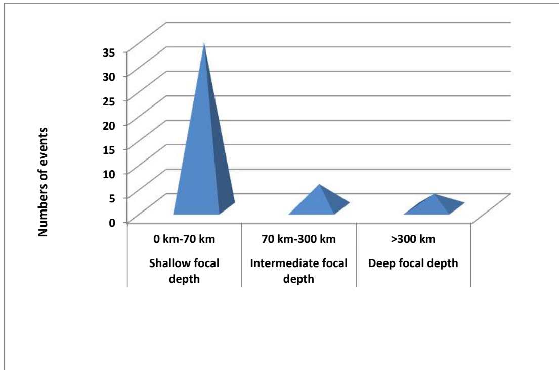
Figure2: Frequency analysis of major earthquakes based on focal depth during the month of July, 2019.
