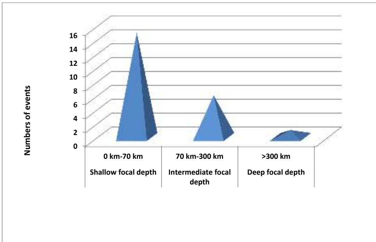
Figure2: Frequency analysis of major earthquakes based on focal depth during the month of December, 2019.
