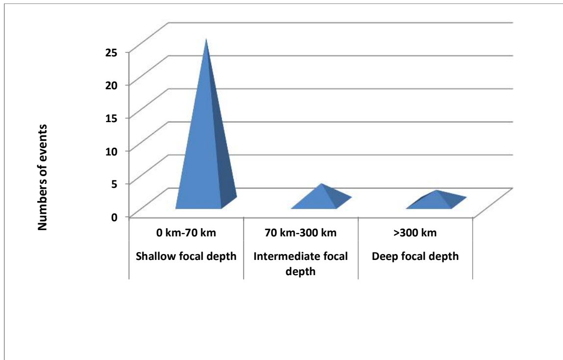
Figure2: Frequency analysis of major earthquakes based on focal depth during the month of September, 2019.
