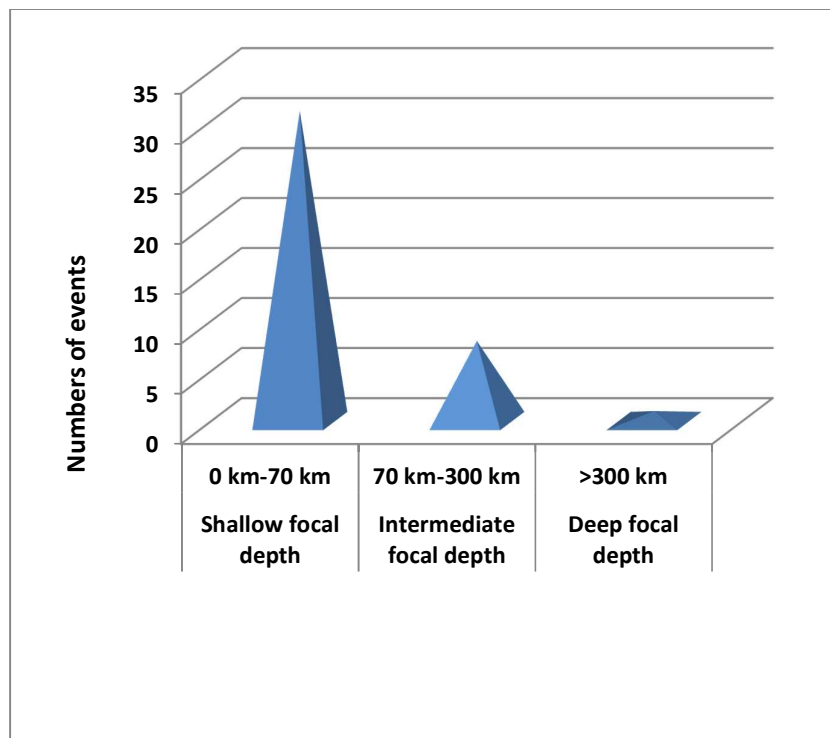
Figure2: Frequency analysis of major earthquakes based on focal depth during February, 2019.
