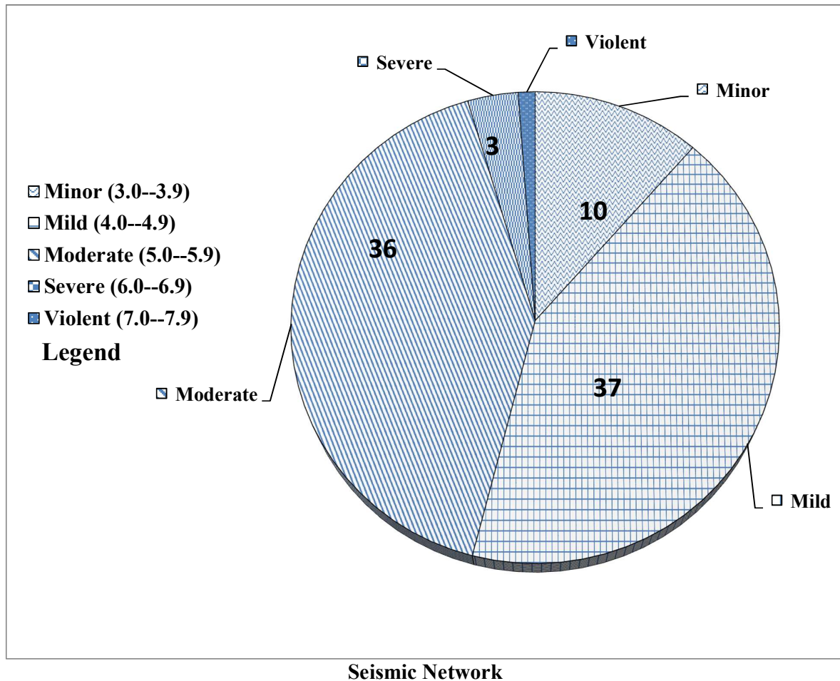
Figure 1: Frequency Analysis of the Magnitude of the Seismic Events Recorded by PMD
